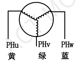
从安装面看为顺时针方向 CLOCKWISE VIEW FROM MOUNTING SIDE
