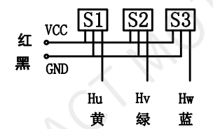
霍尔传感器电源电压+5至+20 VDC HALL SENSOR POWER SUPPLY VOLTAGE +5 TO +20 VDC
